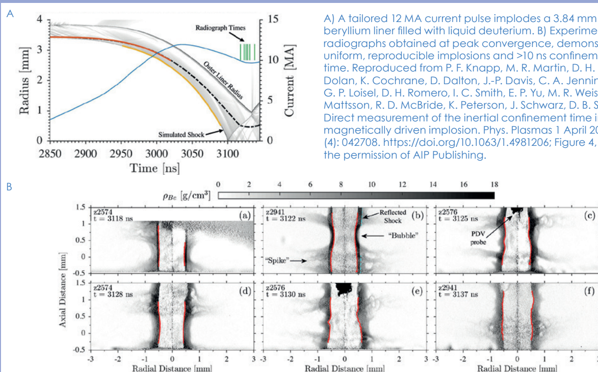
Figure 8: Data from deuterium isentropic compression experiments on Sandia's Z machine.
